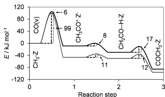
Figure 1. Reaction paths for formation of acetyl from a methyl group and CO within the 12-MR on T1-O4 and the 8-MR on T3-O3. Reaction steps: 0. CO in vacuum, methyl group on the zeolite; 1. acetyl carbocation and negatively charged zeolite; 2. ketene physisorbed onto a Brønsted acid site; 3. acetyl group on zeolite. Black line: reaction steps in the main channel (T1-O4); gray line: reaction steps in the side pocket (T3-O3).
